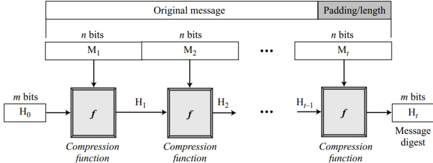
Merkle-Damgård construction
